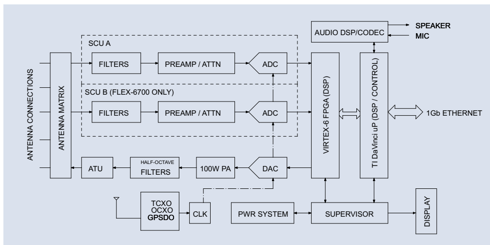
FLEX-6000 Signature Series Hardware Architecture
